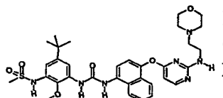
N-[5-tert-Butyl-2-methoxy-3-(3-{4-[2-(2-morpholin-4-yl-ethylamino)-pyrimidin-4-yloxy]-naphthalen-1-yl}-ureido)-phenyl]-methanesulfonamide;
